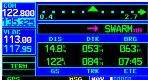
Figure 6-21 Missed Approach Holding Point
