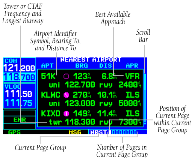
Figure 8-9 Nearest Airport Page
