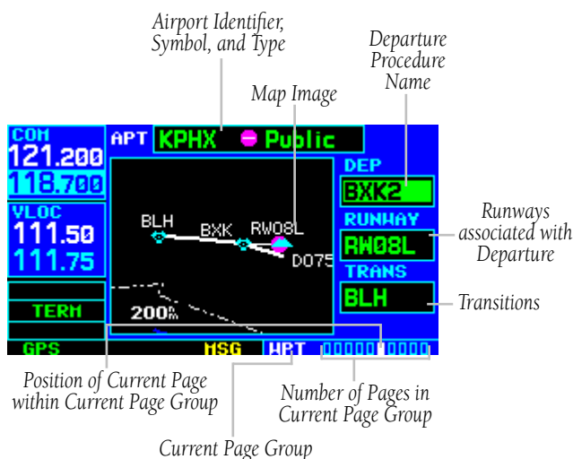
Figure 7-27 Airport Departure Page
