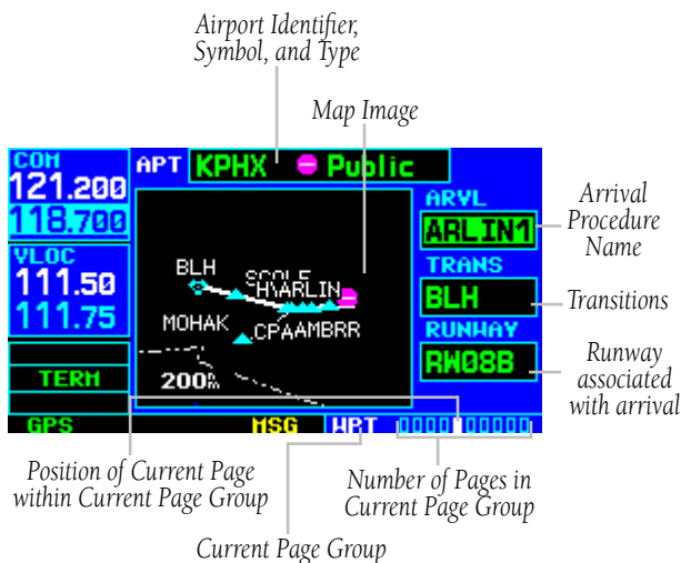
Figure 7-22 Airport Arrival Page
