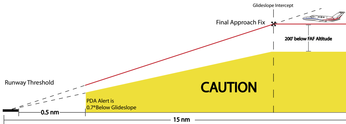
Figure 11-9 ILS Approach PDA Alert Threshold
