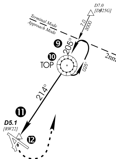
Figure 6-44 Approach Mode
