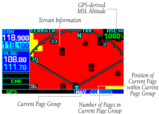
Figure 3-26 TERRAIN Page
