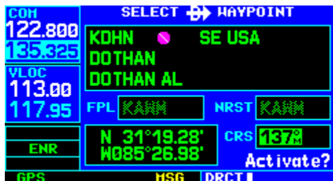
Figure 4-13 CRS (Course) Field Highlighted
