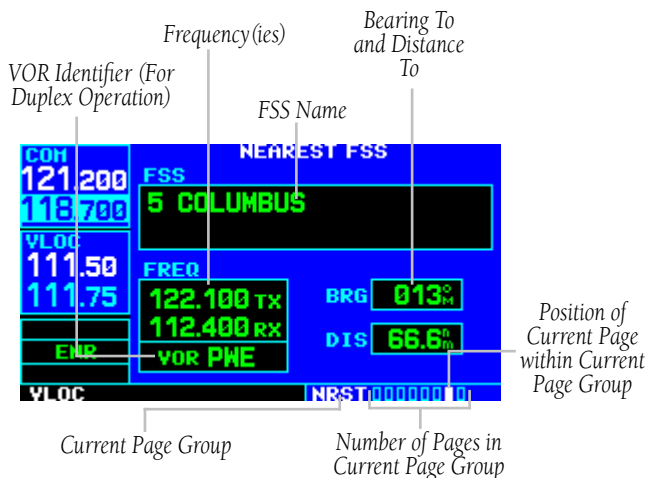
Figure 8-22 Nearest FSS Page
