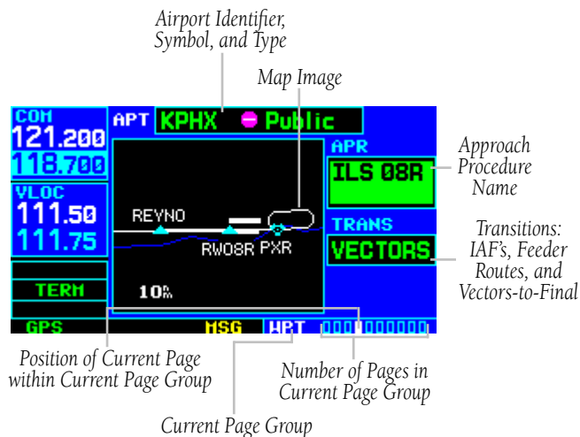
Figure 7-17 Airport Approach Page
