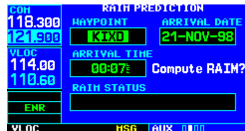
Figure 10-43 RAIM Prediction Page
