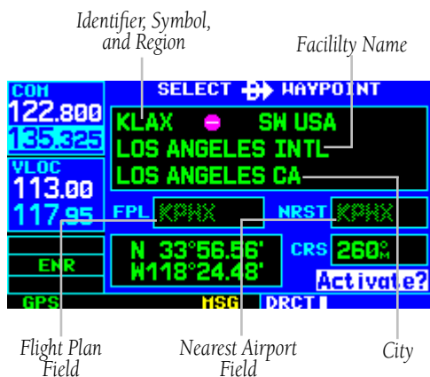
Figure 4-4 Select Direct-to Waypoint Page
