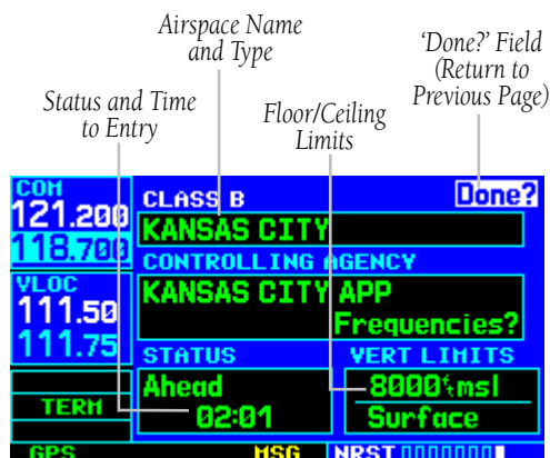
Figure 8-31 Airspace Page
