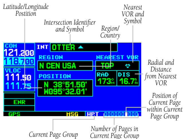
Figure 7-31 Intersection Page
