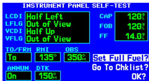
Figure 1-7 'Set Full Fuel?' Highlighted
