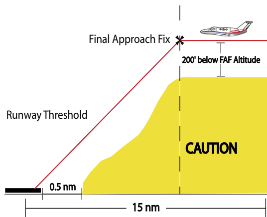
Figure 11-8 Non-Precision Approach PDA Alert Threshold
