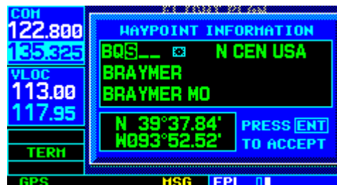
Figure 5-5 Waypoint Identifier Field Selected
