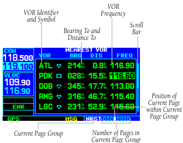
Figure 8-16 Nearest VOR Page
