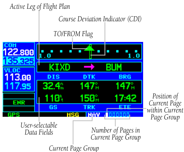
Figure 3-3 Default NAV Page
