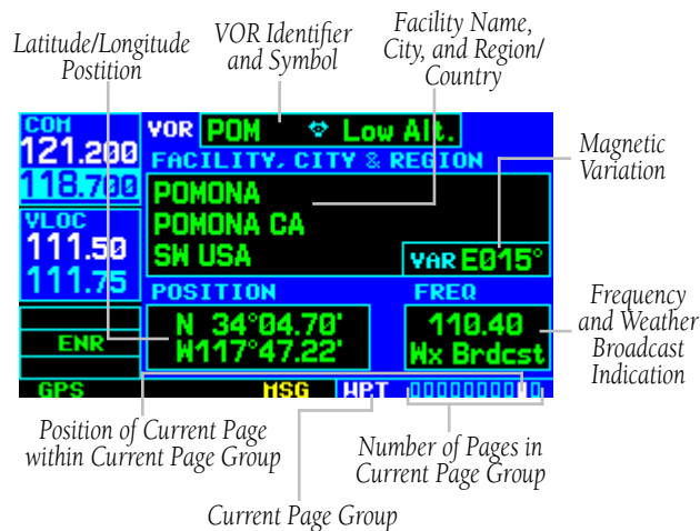
Figure 7-33 VOR Page
