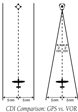
Figure D-8 CDI Comparison
