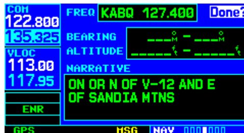
Figure 3-37 Restriction Information Page
