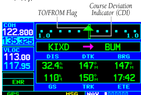
Figure 1-17 Default NAV Page
