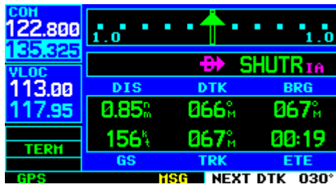
Figure 6-79 Waypoint Alert
