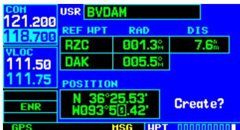
Figure 7-40 Present Position Field Selected
