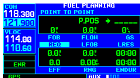
Figure 10-12 REQ Highlighted
