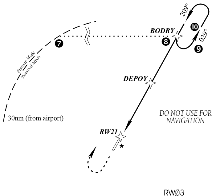
Figure 6-29 Terminal Mode
