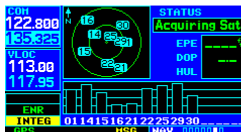
Figure 3-47 Hollow Signal Strength Bars
