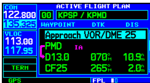
Figure 6-59 Active Flight Plan Page
