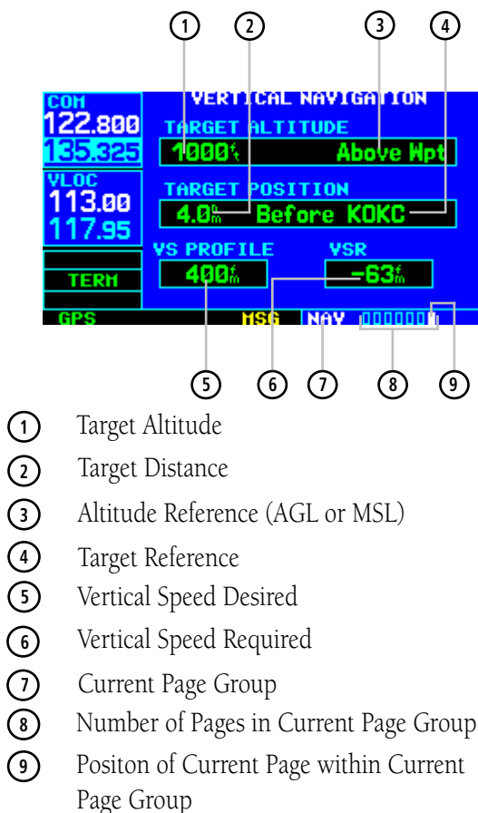
Figure 3-48 Vertical Navigation (VNAV) Page
