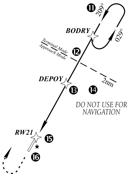
Figure 6-32 Approach Mode
