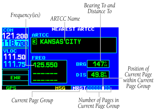
Figure 8-19 Nearest ARTCC Page
