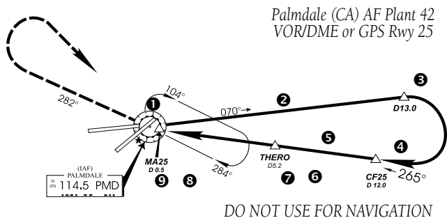
Figure 6-60 KPMD Approach
