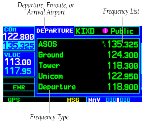
Figure 1-20 NAV/COM Page
