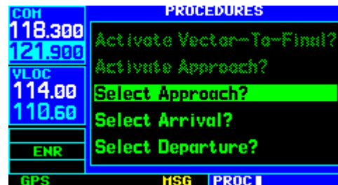
Figure 9-7 Procedures Page
