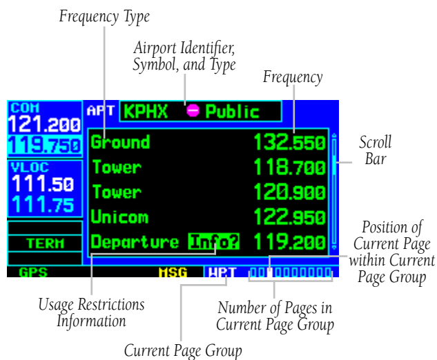
Figure 7-12 Airport Frequency Page
