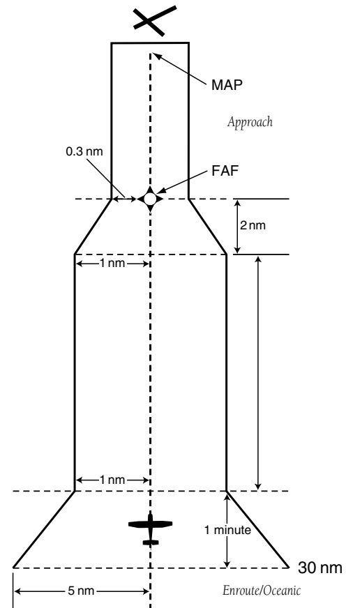
CDI Scale Transition
