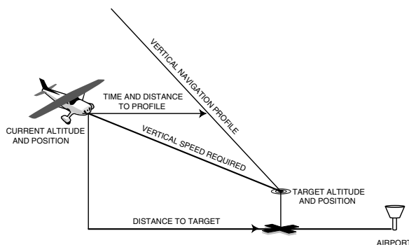
Figure 3-49 Vertical Navigation Profile
