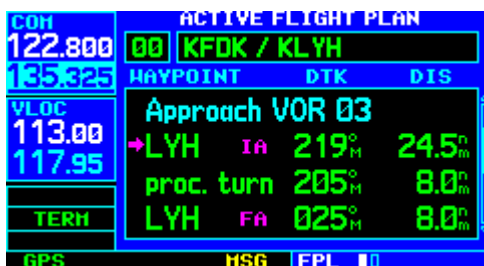
Figure D-2 Active Flight Plan Page
