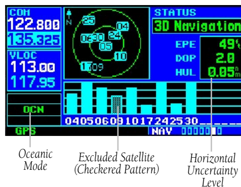
Figure 12-1 Satellite Status Page
